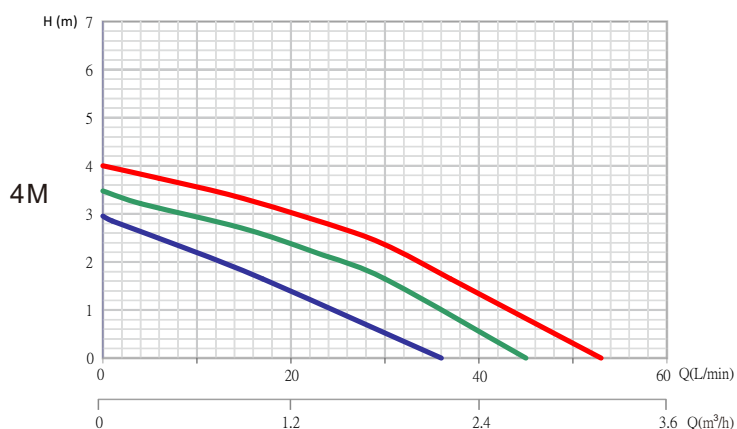
Performance curves
